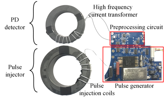
FIGURE 4 Components of the hybrid sensor.
