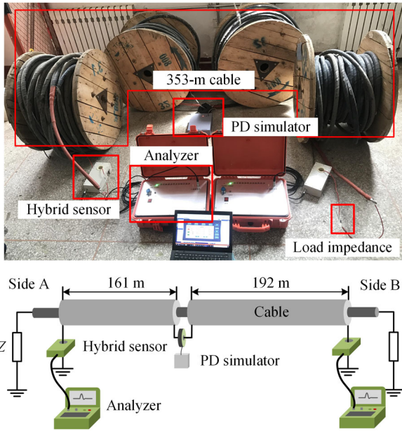
FIGURE 7 Layout of the testing platform.
