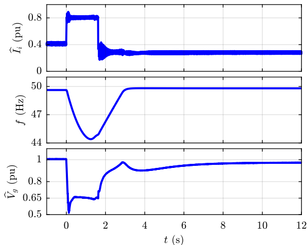
Fig. 21. Results of Test 4. From top to bottom: inverter current amplitude \hat{i}_i (pu); S-VSC frequency f (Hz); capacitor voltage amplitude \hat{V}_g (pu).
