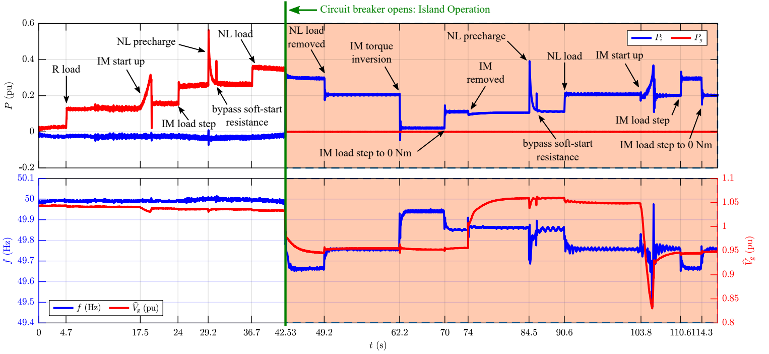
Fig. 15. Results of Test 2: (top) inverter power P_i (pu) and grid power P_g (pu) moving average trends; (bottom) S-VSC frequency f (Hz) and voltage amplitude \hat{V}_g (pu) trends.
