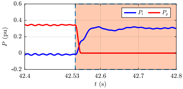
Fig. 16. Transition from grid-mode to island operation in Test 2: inverter power P_i (pu) and grid power P_g (pu) moving average trends.
