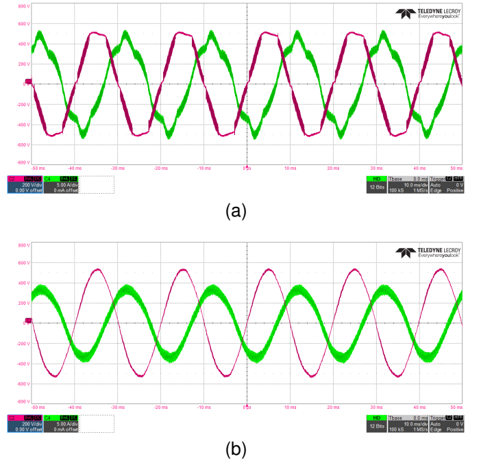
Fig. 17. Line to line voltage v_{g,ab} and current i_{fg,a} waveforms during island operation: (a) with all loads connected; (b) without the NL load.
