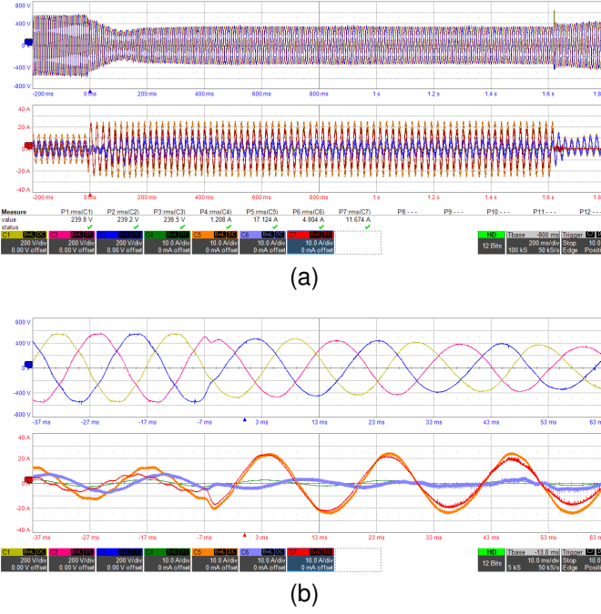
Fig. 20. Results of Test 4. C1, C2 and C3 are the line to line three phase voltages v_{g,LL} . C4 is the R load current i_{R,a} , C5 is the inverter current i_{i,a} , C6 is the IM current i_{IM,a} and C7 is the fault current i_{F,a} . The RMS values are calculated in the time range from 200 ms to 1.6 s. From top to bottom: (a) entire fault; (b) zoom at the beginning of the fault.
