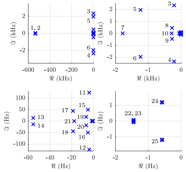
Fig. 6. Eigenvalues map of the system in grid-connected operation.
