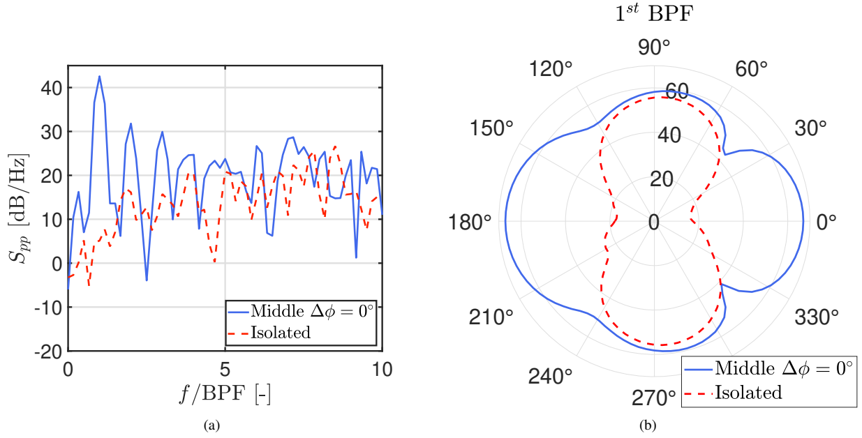
Fig. 9 (a) Far-field noise power spectral density S_{pp} , with microphone position at X = -10D and Y = Z = 0 ; comparison between the distributed middle propeller with \Delta\phi = 0^\circ against the isolated one. (b) Far-field sound L_p directivity plot comparing the distributed middle propeller with \Delta\phi = 0^\circ and the isolated one.
