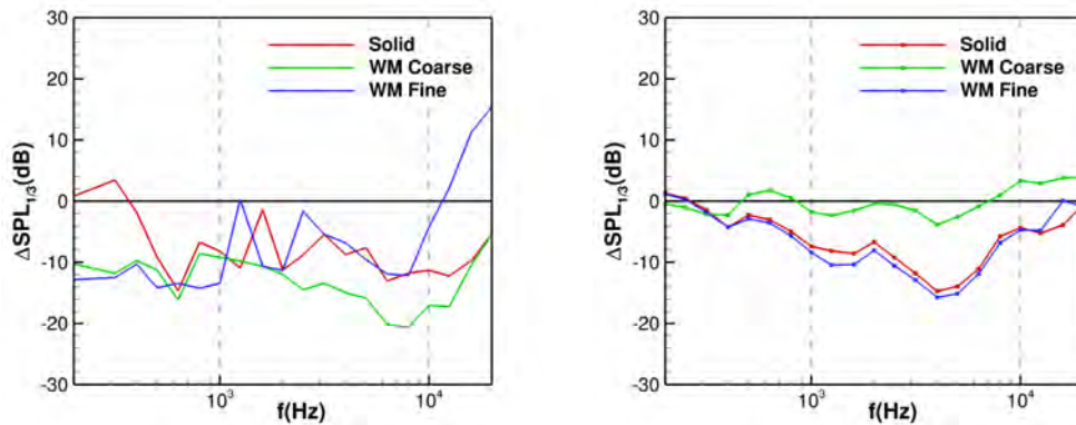
Fig. 24 Sound pressure level difference with respect to the baseline configuration (third-octave band dB, p_{ref} = 2 \times 10^{-5} Pa). Left: simulation; Right: Experiment.
