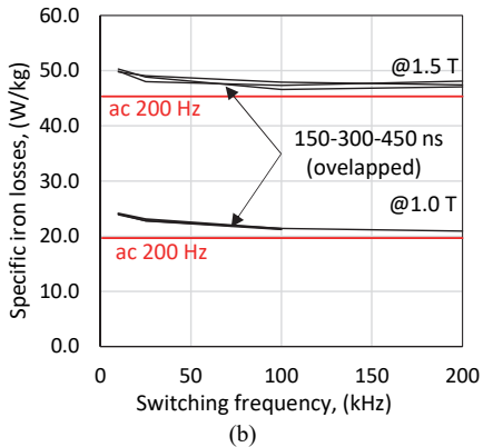
Fig. 5. The switching frequency impact on the iron losses for the FeSi core at 200 Hz: (a) deadtime = 150 ns; (b) 150, 300 and 450 ns.
