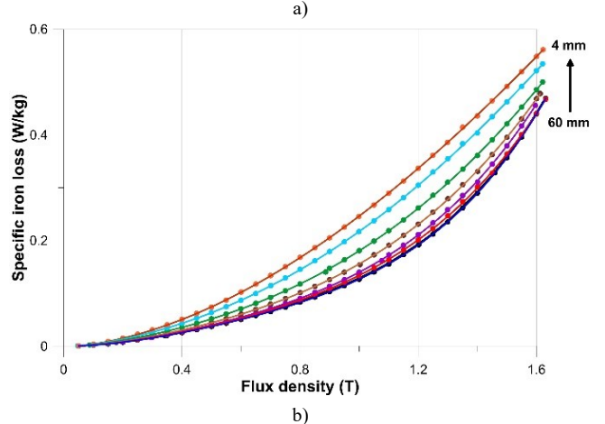
Fig. 2. Measured specific iron loss for M270-35A lamination strips having width in the range 4-60 mm (a) at 50Hz; (b) at 10Hz
