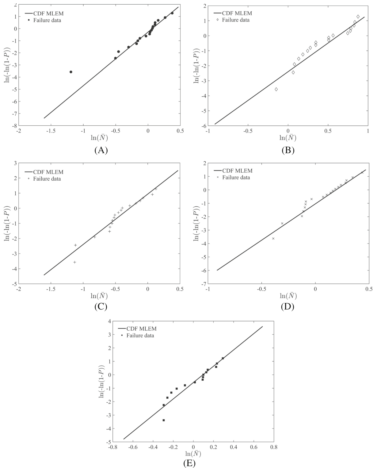
FIGURE 11 Estimated Weibull probability plots for the five different specimen sizes: (A) 3 mm; (B) 6 mm; (C) 12 mm; (D) 24 mm; and (E) 30 mm.
