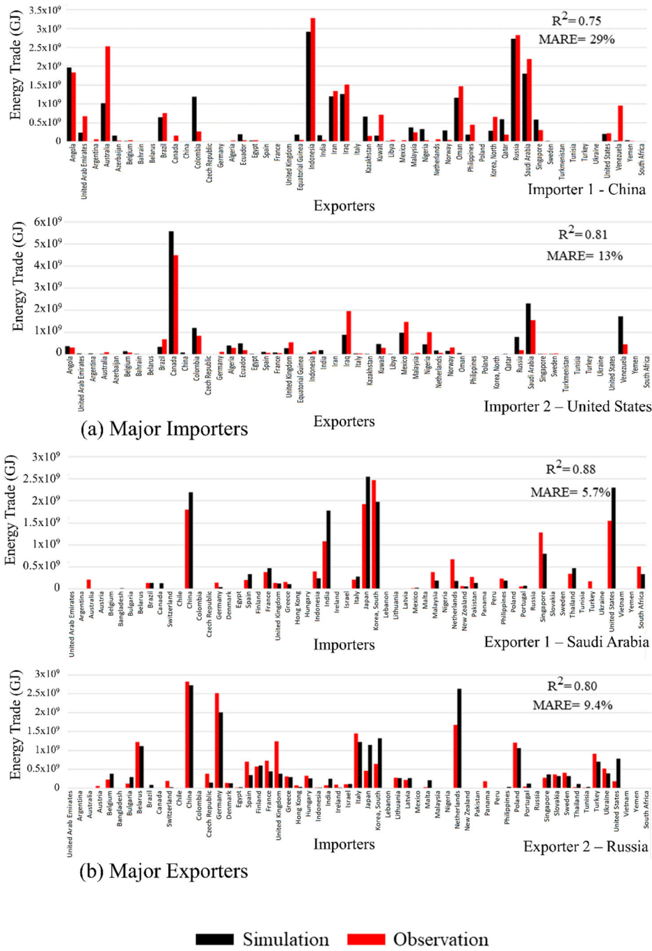
Figure 3. Performance of the RAS method with respect to the simulation of energy flux for (a) two major importers and (b) two major exporters in 2016.
