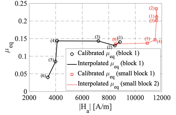
Fig. 5. Permeability values \mu_{eq} for different values of applied magnetic field. In black for large block 1 and red for the small block 2 shown in Fig. 3a.
