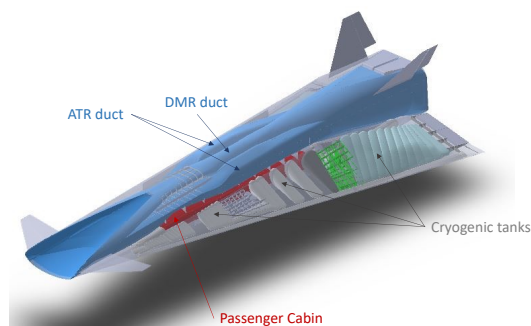
Fig. 1. STRATOFly MR3 vehicle layout and subsystems integration
