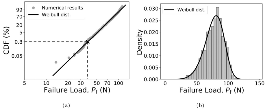
Fig. 16. Weibull distribution of the failure load for the glass beam under three point bending: (a) Linearized cumulative distribution function; (b) Probability density function.
