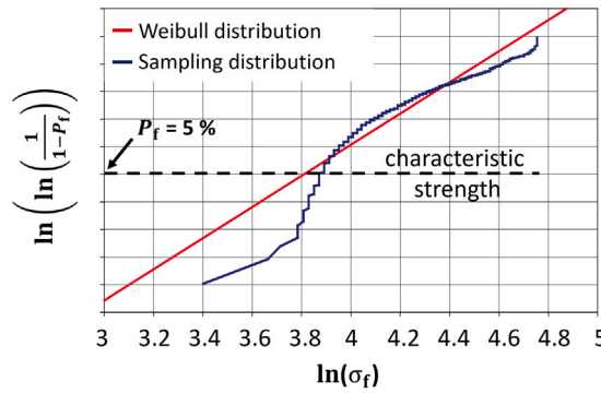
Fig. 1. Cumulative Weibull distribution of the failure stress. Source: Adapted from [13].
