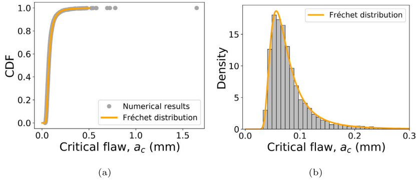
Fig. 12. Fréchet distribution of the critical edge crack size for the glass specimen under uniaxial tensile load: (a) Cumulative distribution function (CDF); (b) Probability density function.
