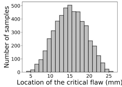
Fig. 22. Location of the critical edge crack for the simply supported beam under uniformly distributed load.
