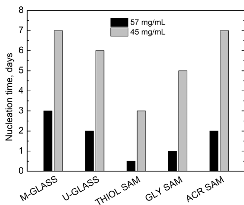
Figure 3. Comparison among the HEWL nucleation times on different surfaces at 57 (black bars) and 45 mg/mL (gray bars) HEWL and 4 wt % NaCl, considering stock solutions.
