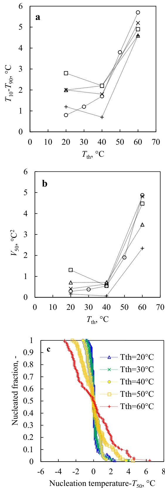
Figure 1. Width of the nucleation temperature distribution ( a : T_{10}-T_{90} , in ^{\circ}\text{C} , b : V_{50} , in ^{\circ}\text{C}^2 ) versus the maximum thawing temperature T_{th} . All the experiments shown in this figure (I–IX in Table 1) are characterized by \tau=9 min. The width of the T_n distributions increases as T_{th} increases from 20 to 60 ^{\circ}\text{C} . In ( a ) and ( b ): circles correspond to experiments I–V, triangles to experiment VI, squares to experiment VII, crosses to experiment VIII, and pluses to experiment IX. c : Nucleated fraction versus nucleation temperature translated by T_{50} (experiments I–V in Table 1). As the maximum thawing temperature rises from 20 to 60 ^{\circ}\text{C} , the survival curves stretch over the horizontal axis, indicating a broader nucleation temperature distribution.
