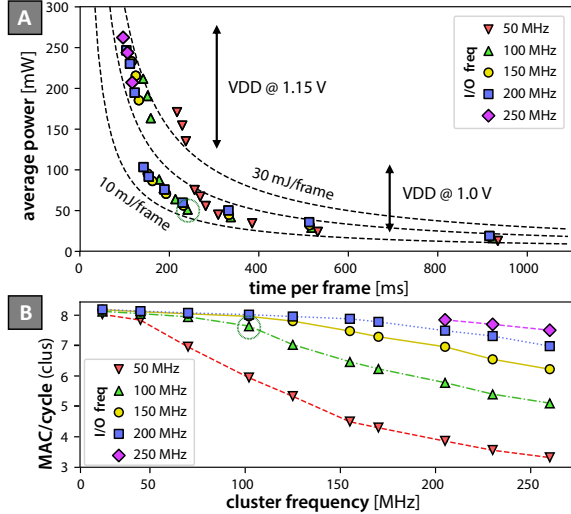
Fig. 10. Power, latency and MAC/cycles performance exploration with sweeping frequencies. The 1.0-MobileNet-128 is used as a benchmark. CL frequency varies in [25 MHz, 260 MHz], I/O one in [50 MHz, 250 MHz]. A green dashed circle highlights the (100 MHz, 100 MHz) configuration that has been used throughout the paper.
