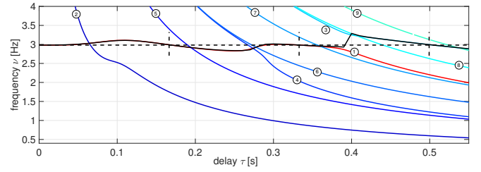
(a) Oscillation frequency \nu .
