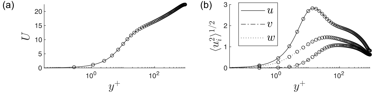
Figure B.6: Mean (a) and root mean square (b) velocity profiles in wall units of the Eulerian phase of the channel flow simulation. Solid lines: present simulation; dots: data from Hoyas and Jiménez (2008) .
