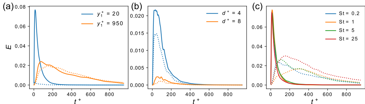
Figure 2: a) Evolution of the encounter probability for pairs of sources at two different wall-normal locations, fixed d^+ = 4 and St^+ = 0.2 (solid lines indicate mixing of streamwise-aligned sources, dashed lines indicate mixing of sources aligned along y ); b) E(t) for source pairs at two different distances, y_1^+ = 100 , St^+ = 0.2 (solid lines indicate mixing of streamwise-aligned sources, dashed lines indicate mixing of sources aligned along y ); c) E(t) for pairs of sources at fixed \mathbf{d} = d\hat{\mathbf{e}}_x , d^+ = 4 and varying Stokes number (solid lines are for source pairs at y_1^+ = 20 , dashed lines at y_1^+ = 950 ).
