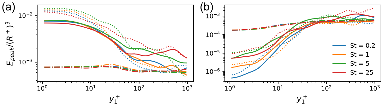
Figure C.7: Streamwise (a) and wall-normal (b) peak encounter probability at varying Stokes number and d^+ = 20 . In all panels, solid lines indicate R^+ = 2 , dotted lines R^+ = 1 , and dash-dotted lines R^+ = 8 (a logarithmic scale is used on the vertical axis).
