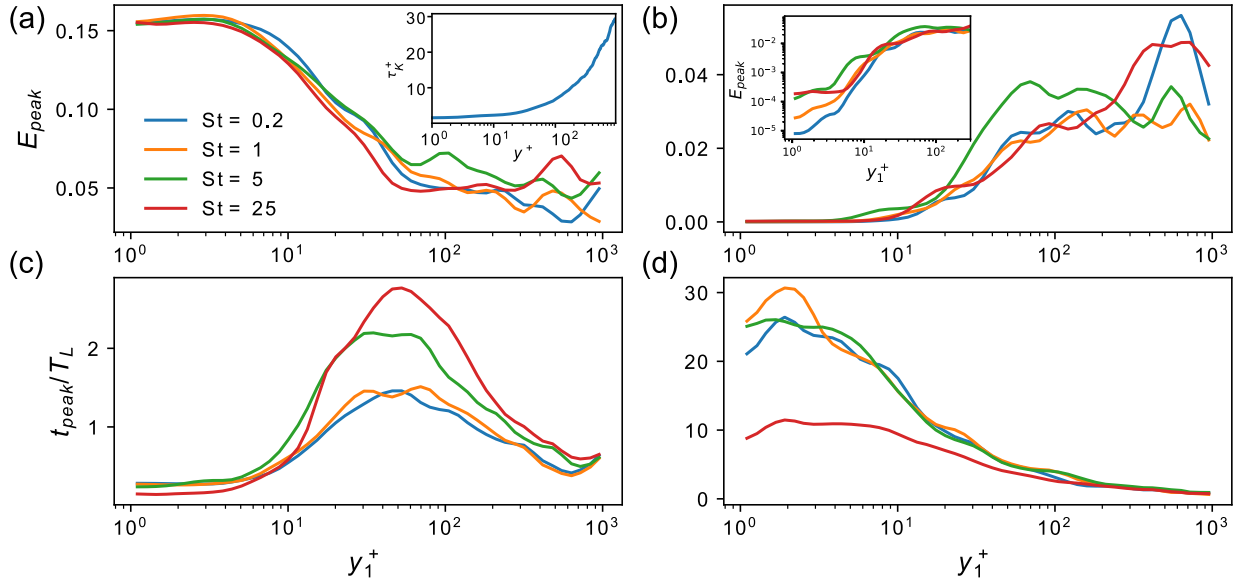
Figure 4: Peak streamwise (a) and wall-normal (b) encounter probability E_{peak} with d^+ = 4 at different Stokes numbers. The inset in the left panel shows the value of Kolmogorov time \tau_p^+ across the channel height, while the inset of the right panel shows a zoom of the data in figure 4(b) with logarithmic vertical axis. Peak time of the streamwise (c) and wall-normal (d) encounter probability t_{peak} with d^+ = 4 at different Stokes numbers.
