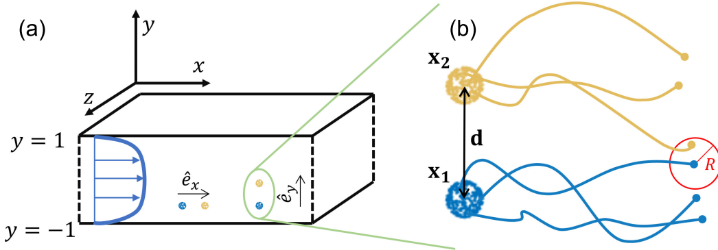
Figure 1: a) Channel geometry and coordinate system; two pairs of sources are represented, one aligned along the streamwise direction, the other along the wall-normal one. b) Schematic depiction of how encounters are determined starting from particle trajectories.
