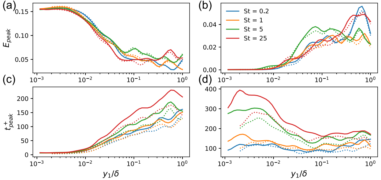
Figure A.5: Streamwise (a) and wall-normal (b) peak encounter probability at \text{Re}_\tau = 950 (solid lines) and \text{Re}_\tau = 590 (dotted lines). d^+ = 4 in all cases. Peak time of the streamwise (c) and wall-normal (d) encounter probability at \text{Re}_\tau = 950 (solid lines) and \text{Re}_\tau = 590 (dotted lines).
