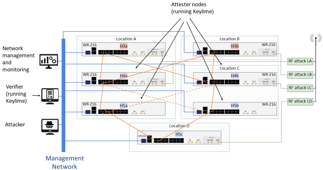
FIGURE 5. Testbed description.
