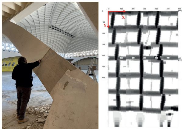
Figure 6 | Rebar survey using pacometer.
