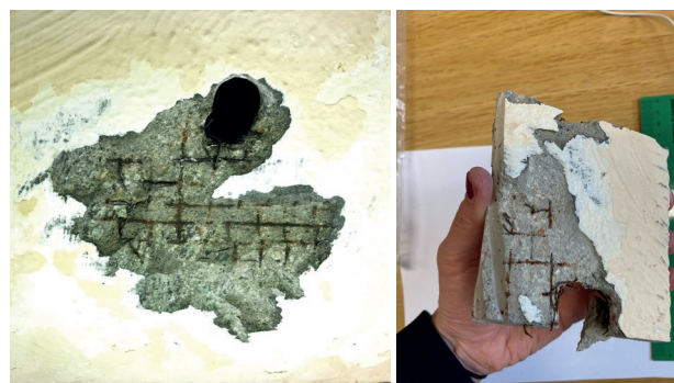
Figure 11 | Sample in the portion of the arch presumably made with Type 680 concrete (on the left), and a sample in the portion of the arch presumably made with Type 500 concrete.
