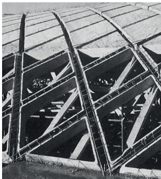
Figure 3 | Detail of the site during the construction phase of the ribbed pavilion vault. In the image it is possible to see the hollows for the casting of the ribs. Università di Firenze, Biblioteca di Scienze Tecnologiche (BST) - Archivi di Architettura, Fondo Pier Luigi Nervi (024-2783).
