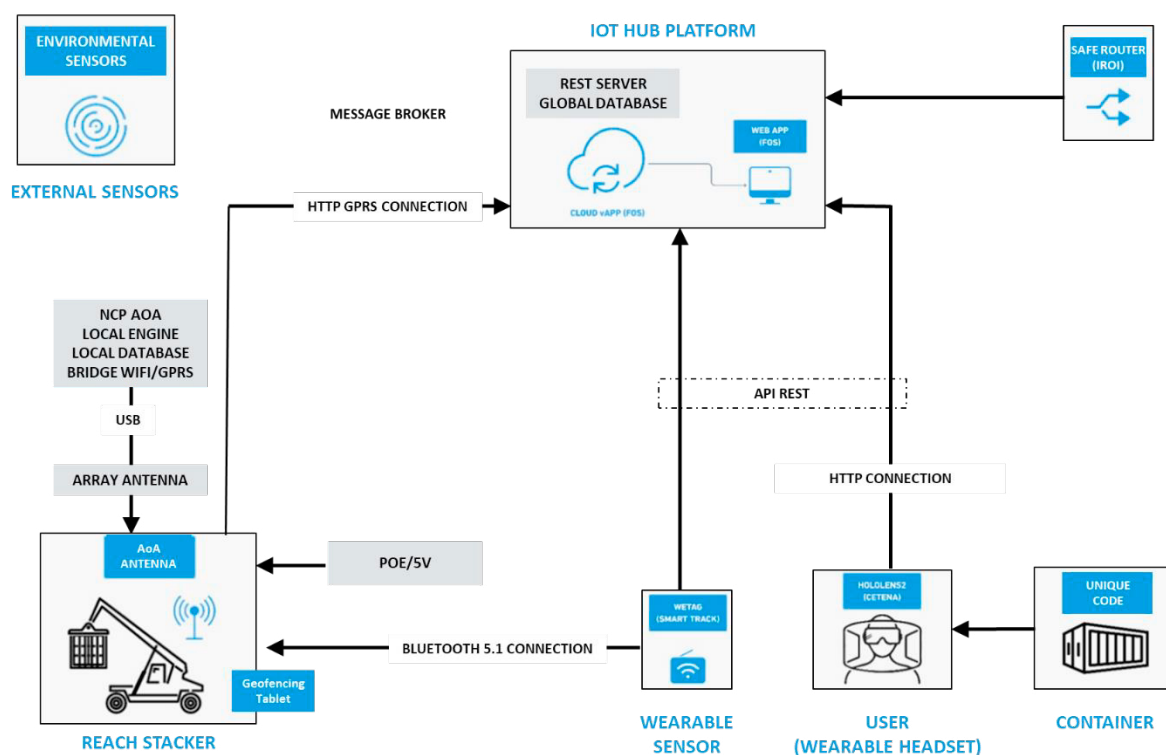
Fig.1. System architecture
