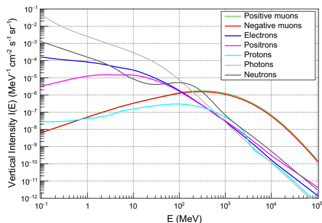
Fig. 6 Differential vertical intensity of secondary cosmic rays at sea level as a function of the energy at (45° N 15° E) Earth Position and on August 1, 2018, computed using the PARMA model as described in the text. The contributions from the various particle species are plotted
