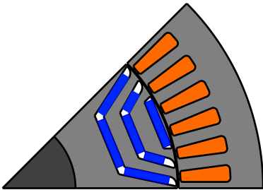
Fig. 2. PM-SyR motor example similar to the reference design. The ferrite magnets are highlighted in blue.
