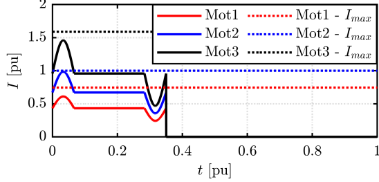
Fig. 13. Current required over the duty cycles and inverter current limits.
