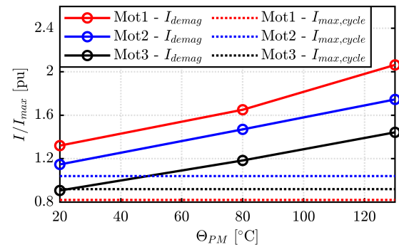
Fig. 12. Demagnetizing currents vs PM temperature. Dashed lines indicate the maximum current requested over the duty cycles. Note that here 1pu corresponds to the maximum inverter current of each motor.
