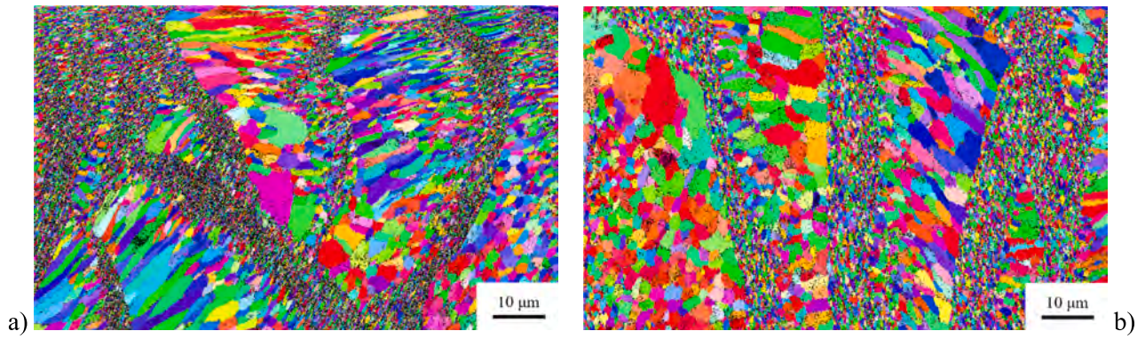
Fig. 6. EBSD images of Scalmaalloy® a) before and b) after aging heat treatment.
