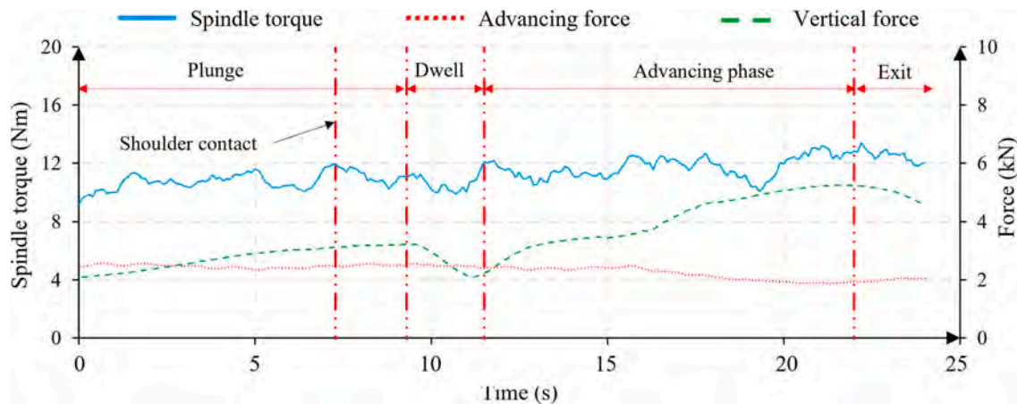
Fig. 4. Monitored spindle torque, advancing and vertical forces during the FSW of Scalmarloy®.
