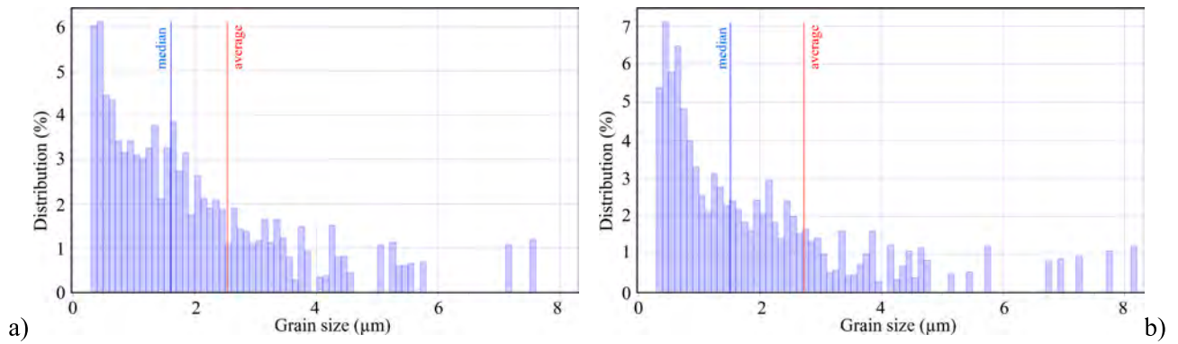
Fig. 7. Grain size distribution (measured according to ASTM E2627 [28]) of Scalmaalloy® a) before and b) after the aging heat treatment.
