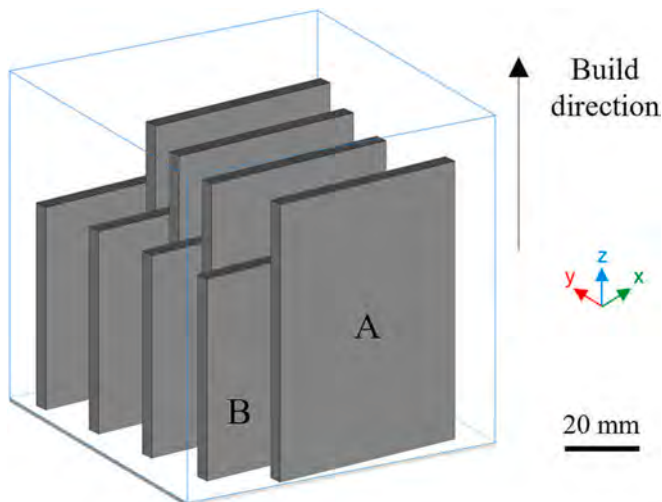
Fig. 1. The two printed orientations of the Scalmaalloy® plates used in the FSW tests.
