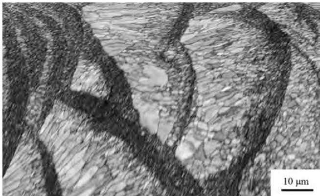
Fig. 5. Lenticular microstructure of the as-printed Scalmaalloy®.
