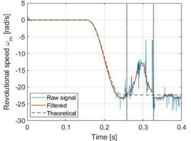
Figure 8 – Revolutions speed of the selected sphere.
