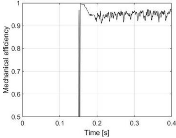
Figure 5 – Mechanical efficiency.
