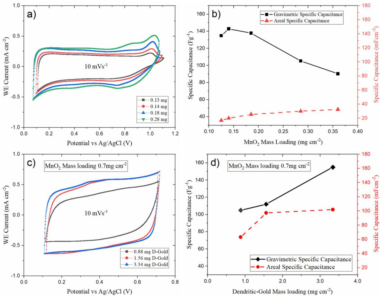
Fig. 6 (a) CV curves of MnO 2 loaded on to flat gold film, with different MnO 2 mass loading, at a scan rate of 10 mV s -1 . (b) Gravimetric and areal capacitance performance in function of MnO 2 mass loading. (c) CV curves of MnO 2 deposited on D-Gold Current collector, varying mass loading of D-Gold, at a scan rate of 10 mV s -1 . (d) Gravimetric and areal capacitance performance in function of D-Gold mass loading, with a fixed amount of MnO 2 0.7 mg cm -2 .
