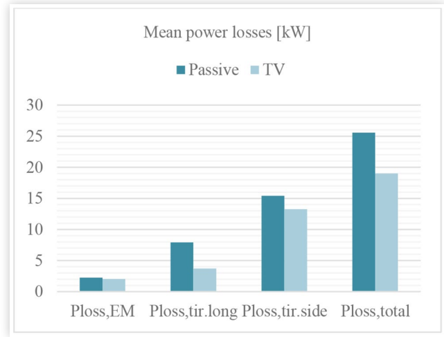
FIGURE 5 Mean Power losses in SRS 100 km/h (dry) maneuver.
