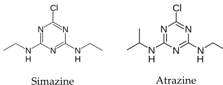
Scheme 2. The chemical structures of simazine (IUPAC name: 6-chloro-N 2 ,N 4 -diethyl-1,3,5-triazine-2,4-diamine) and atrazine (IUPAC name: 6-Chloro-N 2 -ethyl-N 4 -(propan-2-yl)-1,3,5-triazine-2,4-diamine).
