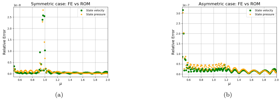
Figure 27. The \mu -dependent error with \bar{N} = 20 and \alpha = 0.01 for symmetric and asymmetric profile of the state variable in (a) and (b) for Distributed control, respectively.
