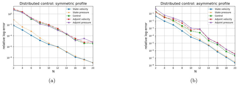
Figure 26. Average error over \mu with \bar{N} = 20 and \alpha = 0.01 for symmetric and asymmetric profile in (a) and (b) for Distributed control, respectively.
