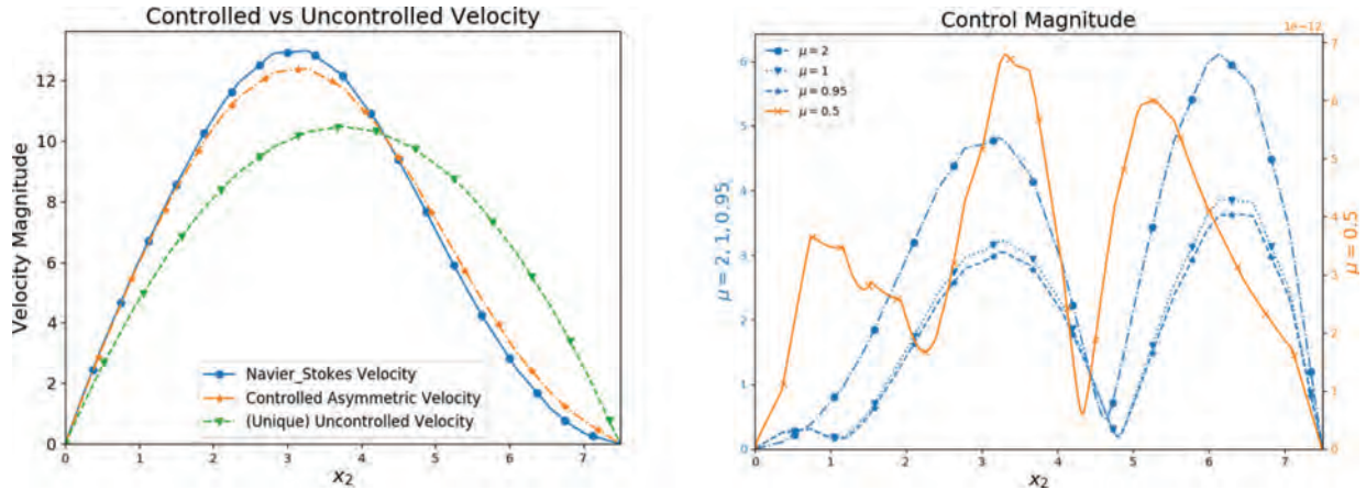
FIGURE 12. Distributed Control : Left: comparison of velocity profiles in the controlled and uncontrolled cases for \alpha = 0.01 , \mu = 2 on \Gamma_{\text{obs}} w.r.t. the asymmetric desired profile when following the natural optimal branch. Right: representation of control variable evolution for \alpha = 0.01 , \mu = 2, 1, 0.95, 0.5 for x_1 = 45 when following the natural optimal branch.
