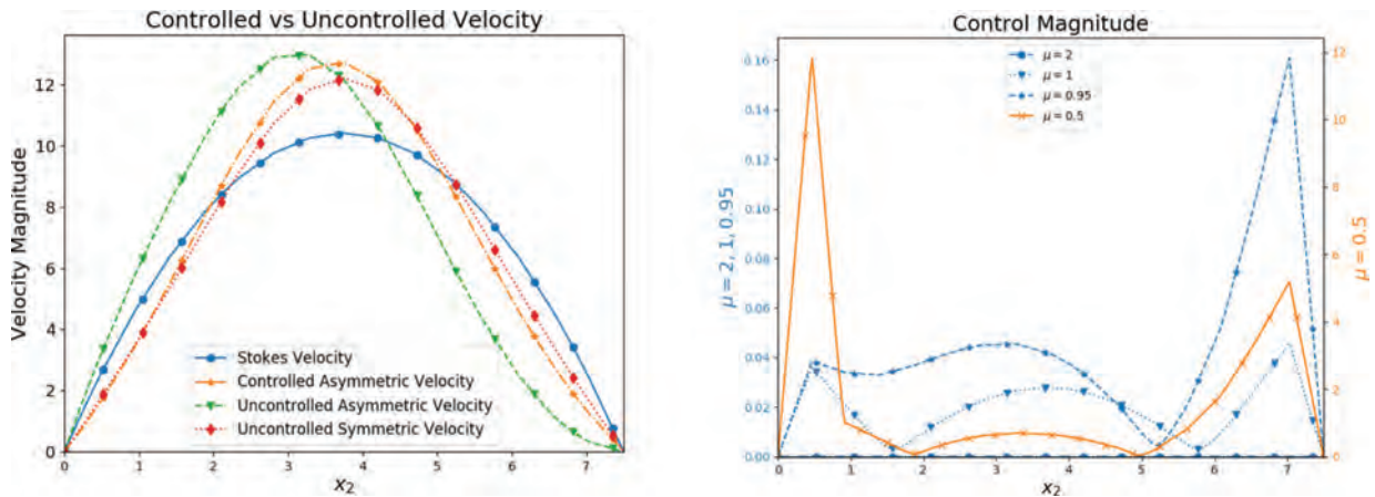
FIGURE 7. Neumann Control : Left: comparison of velocity profiles in the controlled and uncontrolled cases for \alpha = 0.01 , \mu = 0.5 on \Gamma_{\text{obs}} w.r.t. the desired profile when following the natural optimal branch. Right: representation of control variable evolution for \alpha = 0.01 , \mu = 2, 1, 0.95, 0.5 over \Gamma_{\text{out}} when following the natural optimal branch.
