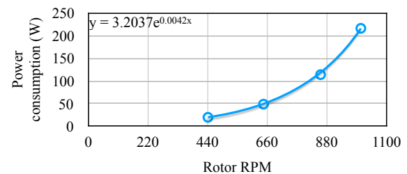
Figure 8. Drone battery power versus motor angular speed [25].
