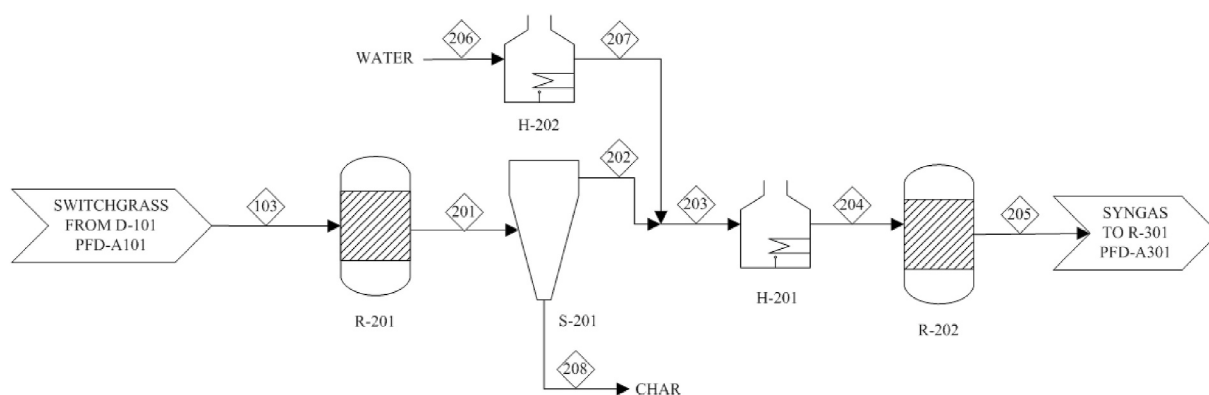
Fig. 3. PFD-A201 Gasification.
