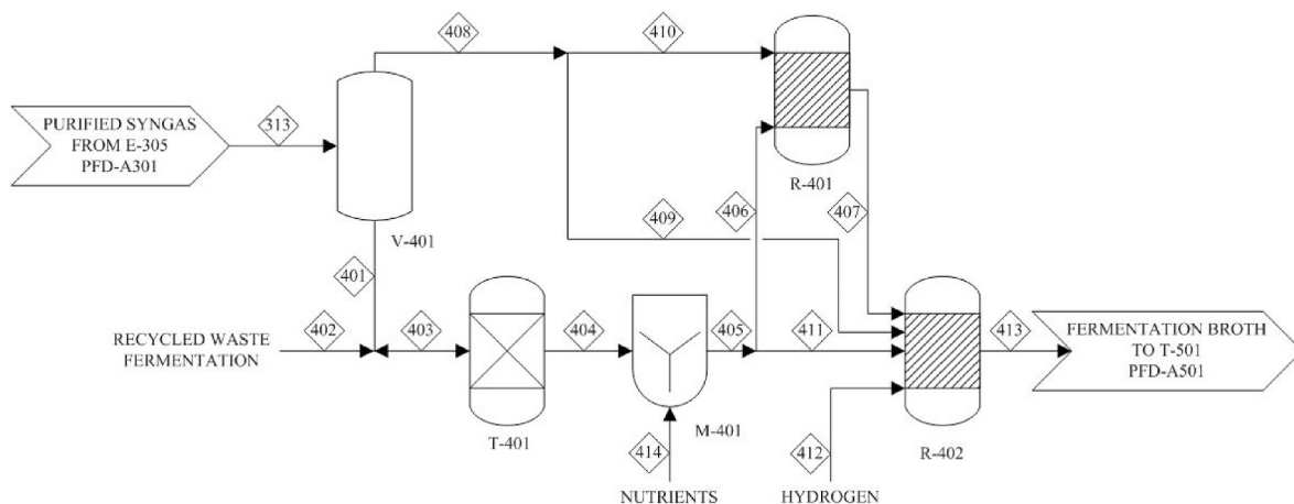
Fig. 6. PFD-A401 fermentation.
