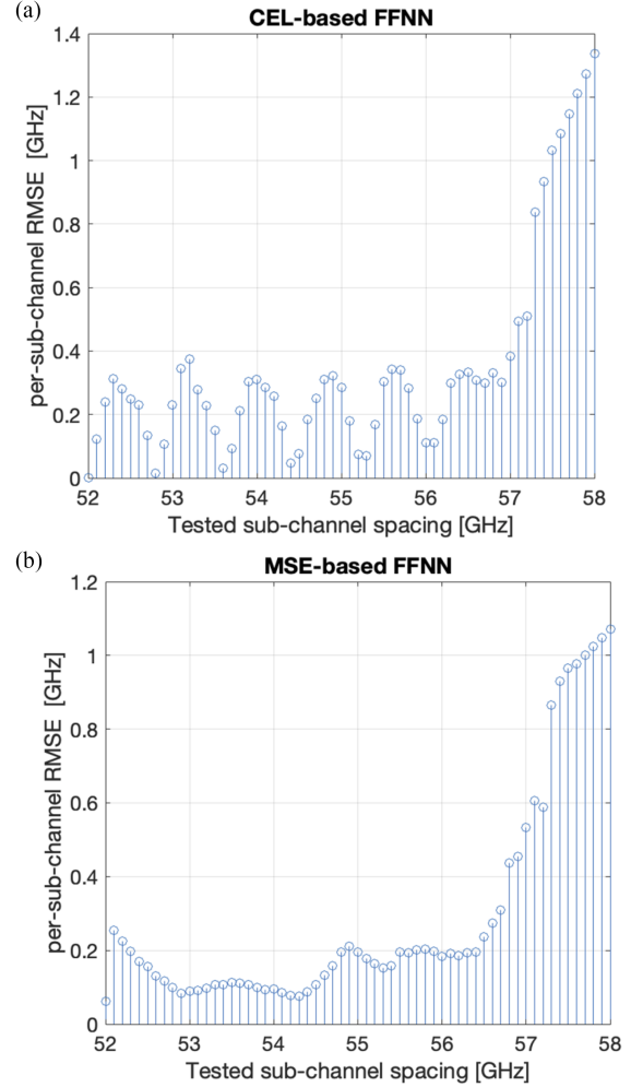
Fig. 5. Root Mean Square Error per tested sub-channel spacing, using simulation test dataset, using CEL-based FFNN (a) and MSE-based FFNN (b).
