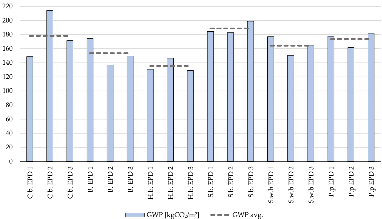
Figure 12. GWP A1-A3|LC for each wall model considered. (C.b. = Concrete block; B. = Bricks; H.b. = Hollow bricks; S.b. = Sandstone bricks; S.w.b. = Shuttering wood chips blocks; P.p = Prefabricate concrete panels).
