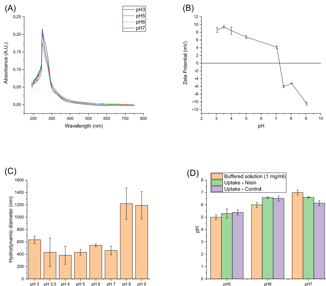
Fig. 4. Characterization of 1 mg/ml nisin solutions by (A) UV-Vis spectroscopy, (B) zeta potential analysis, and (C) hydrodynamic diameter of nisin, measured by DLS analysis, in aqueous solution (1 mM KCl) as a function of pH. (D) pH values of the buffered nisin solutions, nisin uptake solutions, and control uptake solutions (CT soaked in buffered solutions without nisin) at pH5, pH6, and pH7, respectively.
