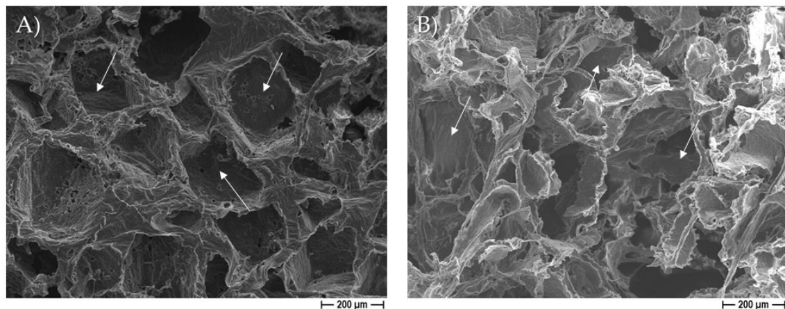
Figure 3. Representative higher magnification FESEM micrographs of PCL samples obtained by adding 30% eugenol EO to the polymer using NaCl (A) or 30% cinnamon oil to the polymer using \text{NaNO}_3 (B) as pore forming salt, showing microporosities within the struts, and on the pore walls (white arrows).
