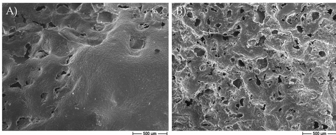
Figure 4. Representative FESEM micrographs of PCL samples obtained by adding 30% eugenol to the polymer using NaCl (A) or \text{NaNO}_3 (B) as pore forming salt, showing the surface microporosities.
