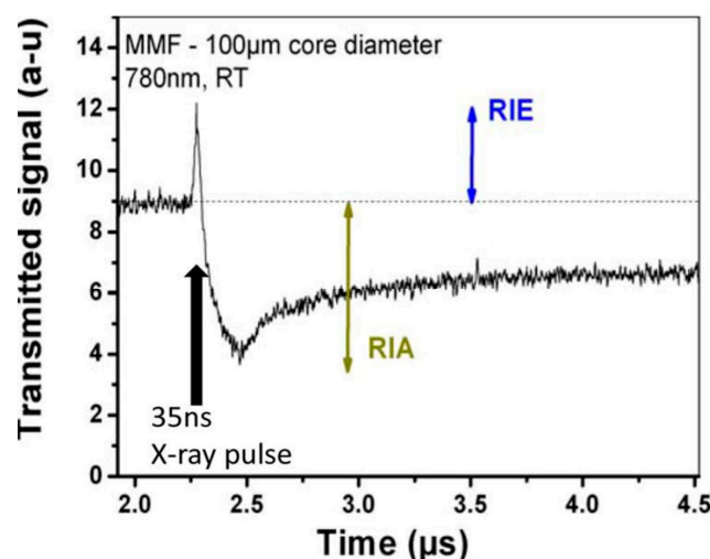
Figure 12. Radiation-induced emission and attenuation of a multimode fiber at 780 \text{ nm} irradiated for 35 \text{ ns} with 1 \text{ MeV} X-rays [102].
