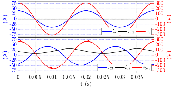
FIGURE 11. IFI-OBC using active zero torque control with magnetizing current on the ZTL for \theta = \pi/6 . Upper plot: current and voltage on grid side of the PMSM. Lower plot: Current and voltage on the battery side.
