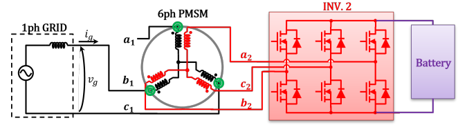
FIGURE 4. Proposed single-phase IFI-OBC topology.
