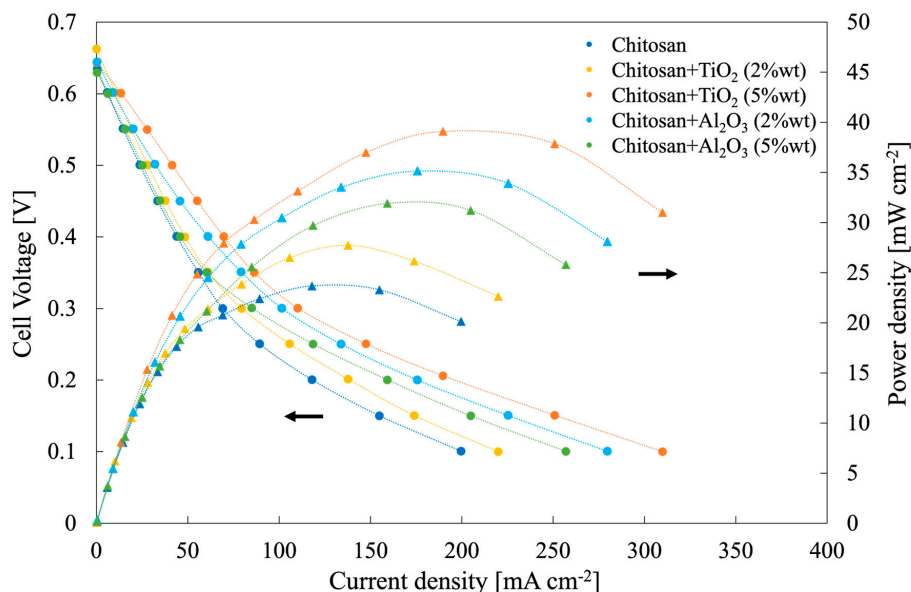
Figure 9. Polarization and power density curves related to a single module DMFC of 1\text{ cm}^2 as active area, employing all the synthesized membranes, operating at 50\text{ }^\circ\text{C} and fed with 2 M methanol aqueous solution at the anode and oxygen at the cathode.
