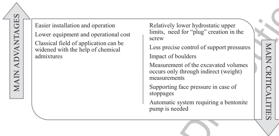
Figure 2.94 Earth Pressure Balance (EPB), summary of main advantages and criticalities.
