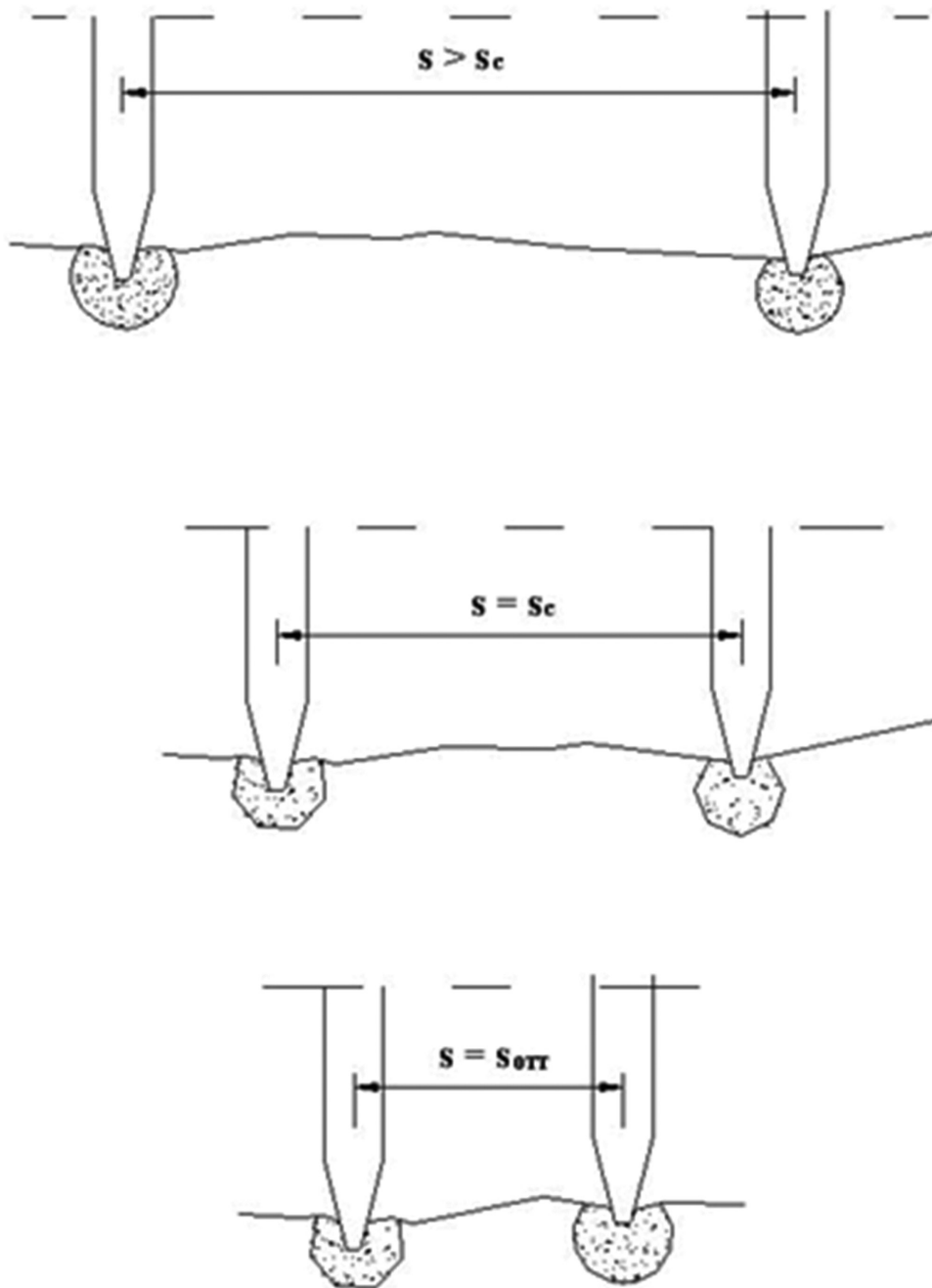
Figure 2.59 Critical and optimal cutters spacing.
