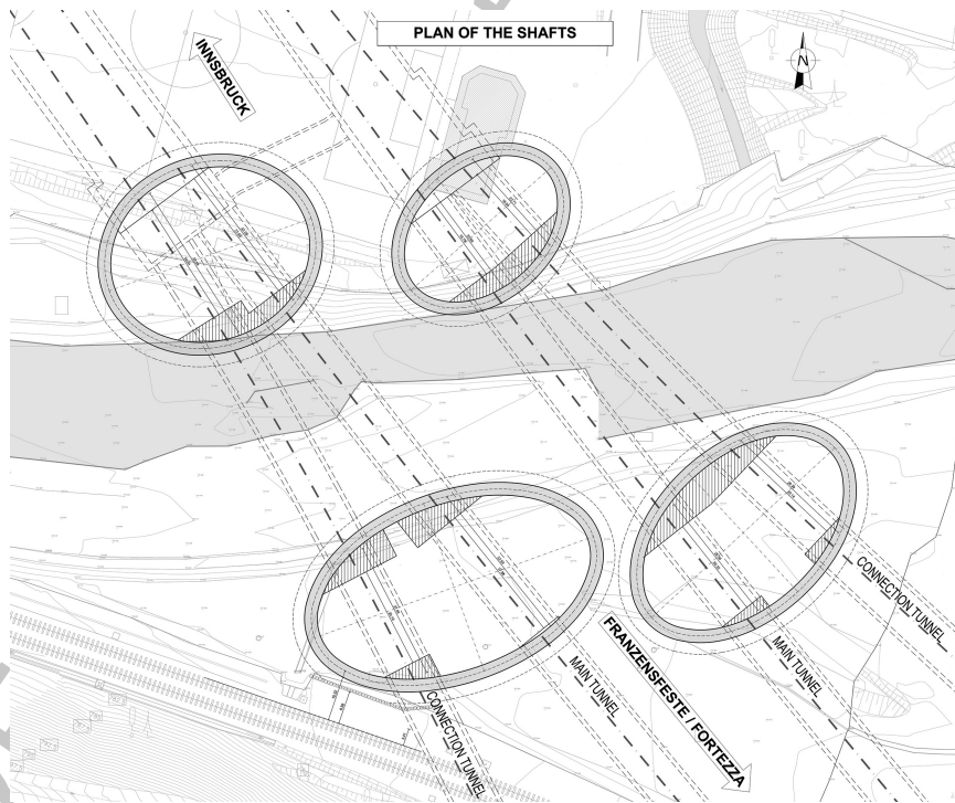
Figure 2.126 Map layout of the four shafts with dotted lines for the four tunnels crossing them (two main tunnels in the middle and two interconnecting tunnels on either side). (Courtesy of BBT SE.)
