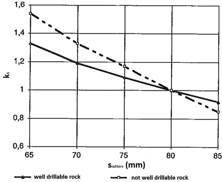
Figure 2.73 Correction factor k_s as a function of the spacing between cutters s_{\text{cutters}} (Gehring, 1995).
