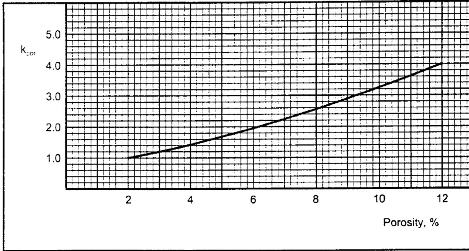
Figure 2.76 Diagram for k_{por} assessment (Bruland, 1998).
