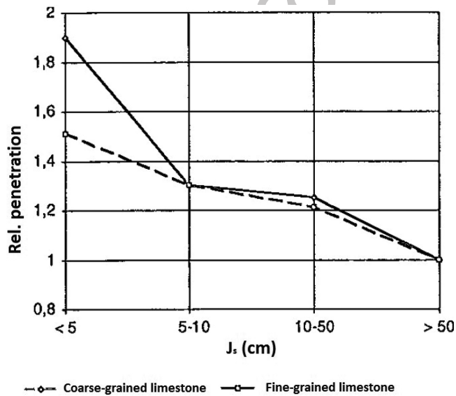
Figure 2.71 Effect of joint spacing J_s (Gehring, 1995).
