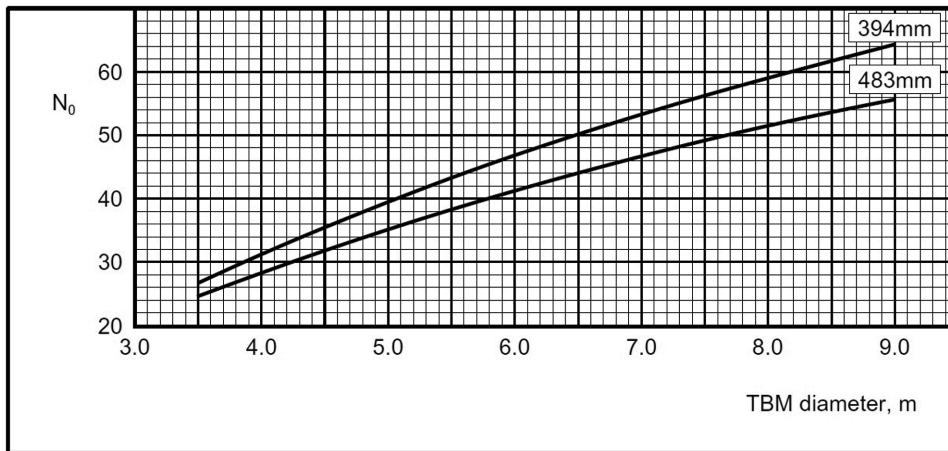
Figure 2.84 Diagram to obtain the average number of cutters for a given \Phi_{\text{TBM}} (Bruland, 1998).
