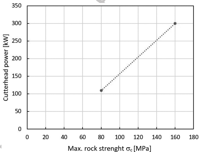
Figure 2.17 Cuttable rock strength as a function of machine weight and cutter head power.
