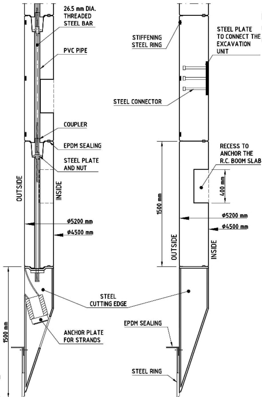
Figure 2.139 Diagram of the precast rings lining, showing connection system, lower segment and cutting edge.
