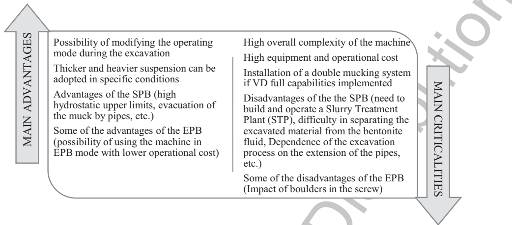
Figure 2.98 Variable density hybrid machines (VD), summary of main advantages and criticalities.
