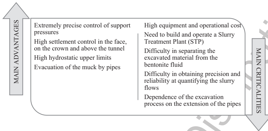
Figure 2.91 Slurry Pressure Balance (SPB), summary of main advantages and criticalities.
