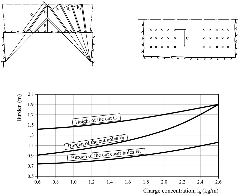
Figure 2.4 Example of calculation of V-cuts charges. The nomogram shows the relationship between the charge concentration l_b and the parameters B_1 , B_2 and C for different drilling diameters and different explosives. (Modified from Olofsson (1991).)
