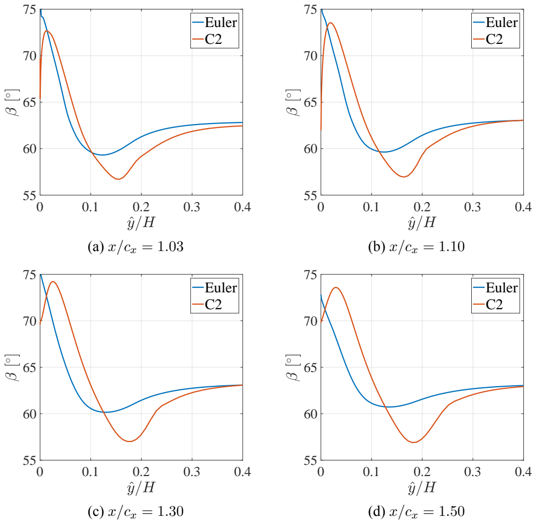
Fig. 9 Comparison of the pitchwise averaged flow angle \beta respect to the axial direction, obtained by solving Euler and RANS equations, along the spanwise direction at four axial locations.
