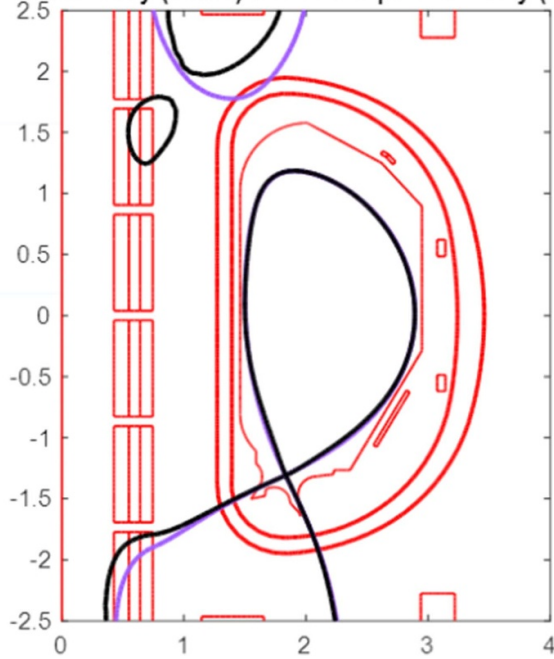
Figure 16. Comparison of the plasma boundary between the starting reference equilibrium calculated by CREATE-NL assuming bellshape plasma profiles (in violet) and the equilibrium recalculated by CREATE-NL in order to obtain the desired magnetic-separatrix shape assuming the JINTRAC plasma profiles (in black).
