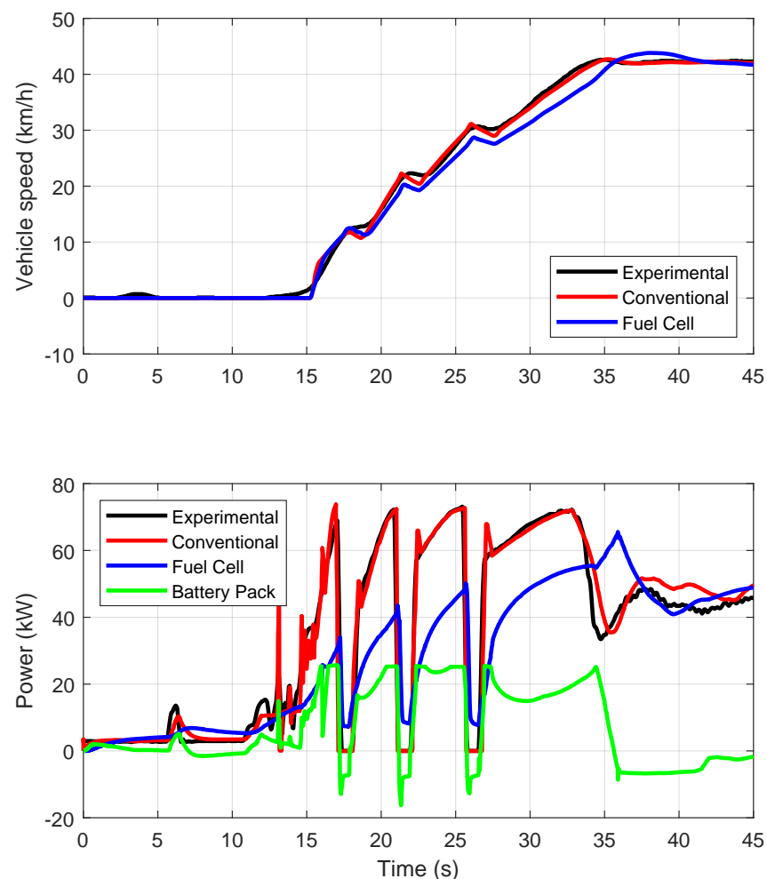
Figure 14. Acceleration test: Experimental vs. Simulations.
