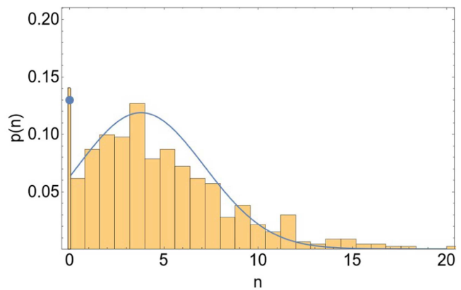
FIG. 1. Representative example of the distribution p(n) of population sizes for v = 0.22 , K = 5 , \sigma_c^2 = a = m = 1 , and \sigma_K^2 = 0 . The solid line is the prediction obtained from (53), the blue marker denoting the weight of the peak at n = 0 (i.e., the fraction of extinct species). Bars represent instead the histogram of the population sizes of 10^3 species obtained by averaging the steady state populations of 100 independent realizations of MacArthur's model (1) and (2).
