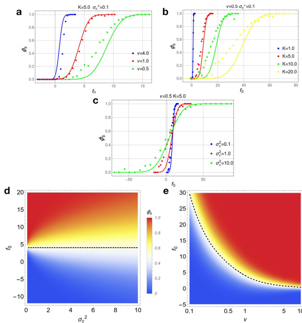
FIG. 5. Panels (a)–(c): Survival probability \phi_s as a function of f_0 for different values of \nu (panel a), K (panel b), and \sigma_c^2 (panel c), with remaining parameters fixed as indicated. (d) Survival probability \phi_s as a function of f_0 and \sigma_c^2 for fixed K = 5 , c = 1 , a = 1 , m = 1 , and \nu = 1 . The dashed line at f_0 = 4 corresponds to \phi_s = 1/2 . (e) Survival probability \phi_s as a function of f_0 and \nu for fixed K = 5 , c = 1 , a = 1 , m = 1 , and \sigma_c^2 = 1 . The dashed line corresponds to \phi_s = 1/2 .
