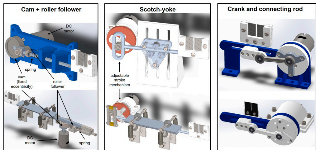
Figure 7. Design of reciprocating mechanisms.
