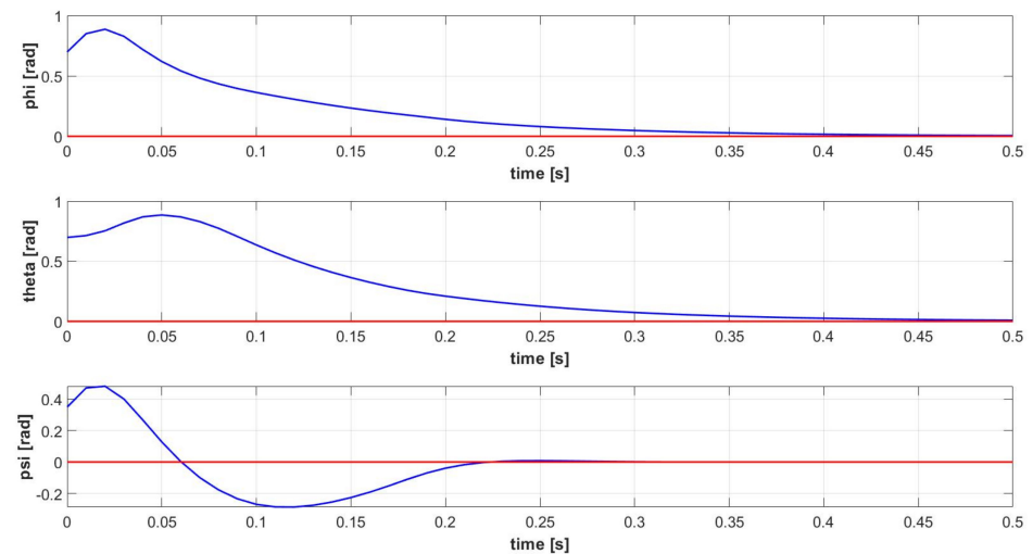
Figure 6. Euler angles signals [\phi(t), \vartheta(t), \psi(t)] of the controlled attitude system (blue): FL-based Attitude Stabilizer (red).
