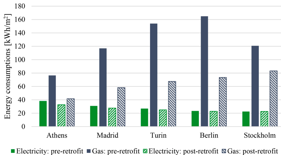
Fig. 6. Simulated electricity and gas consumptions for the five European locations in normal operation, pre- and post-retrofit interventions.
