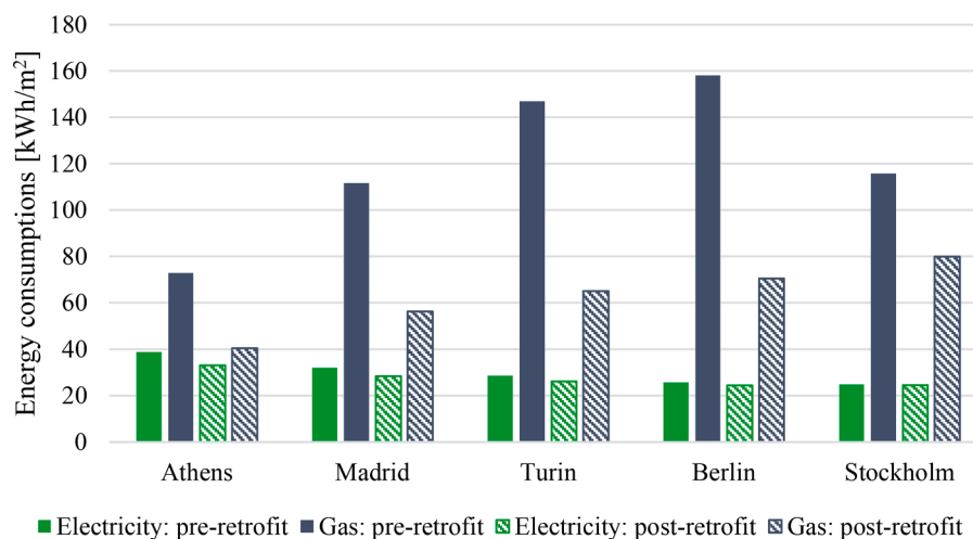
Fig. 7. Simulated electricity and gas consumptions for the five European locations in emergency operation, pre- and post-retrofit interventions.
