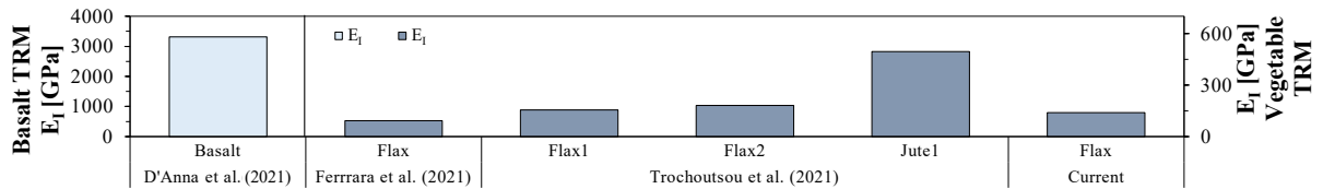
Fig. 7. Comparison of the initial tangential modulus E_t between current experimental and literature results.
