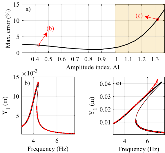
Fig. 9 Frequency response for several forcing input amplitudes, Helmholtz–Duffing oscillator with 3% noise and nonlinear modeling errors. The maximum error on the NFRC is depicted in a . Extrapolation occurs when AI > 1 (yellow region). Black lines in b and c : theoretical results; dashed-dotted red lines in b and c : HBM-NSI result
