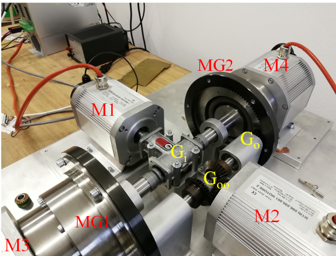
Fig. 36: Picture of the prototype. The motors labels are in accordance to the ones in Fig. 26: here the traction motor M1 is fed, while the other motors are in no load condition.
