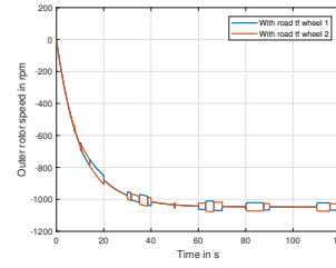
Fig. 17: Wheels speed \omega_{o1} and \omega_{o2} with the time dependent steering radius of Fig. 16.
