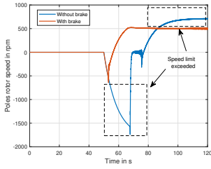
Fig. 14: Poles rotor speed \omega_s with open loop: comparison with and without brake.
