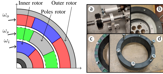
Fig. 1: One fourth of a typical magnetic gear. Materials: magnets (blue-red), ferromagnetic iron (grey), polymeric (green), shaft (black). Fig. 2: Components of the prototyped magnetic gear: (a) inner rotor, (b) outer rotor, (c) poles rotor back and (d) poles rotor front.
