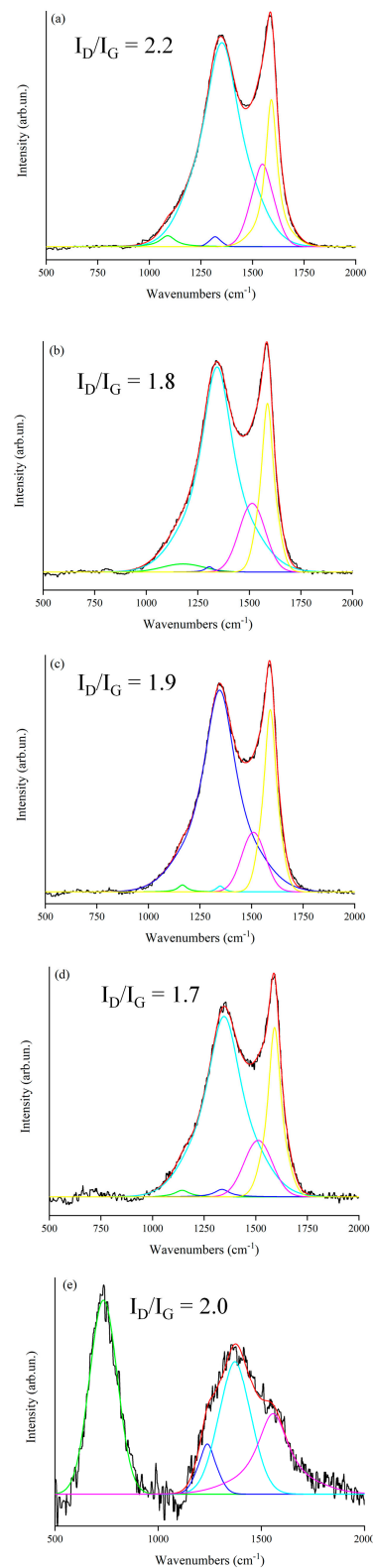
Figure 3. Raman spectra (black lines) in the range from 500–2000 cm -1 of RM-BC materials containing (a) 0 wt., (b) 5 wt.%, (c) 10 wt.%, (d) 20 wt.% and (e) 50 wt.% RM respectively. Fitted signals (red lines) were obtained by using Gaussian-Lorentzian (GauL) or line-shaped components (colored lines), according to Tagliaferro et al. [49].
